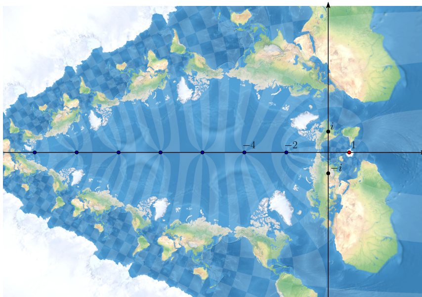
\zeta(s)
